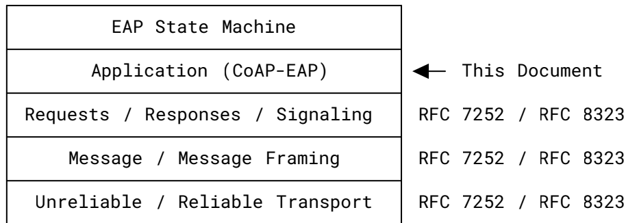
Figure 2: CoAP-EAP Stack
